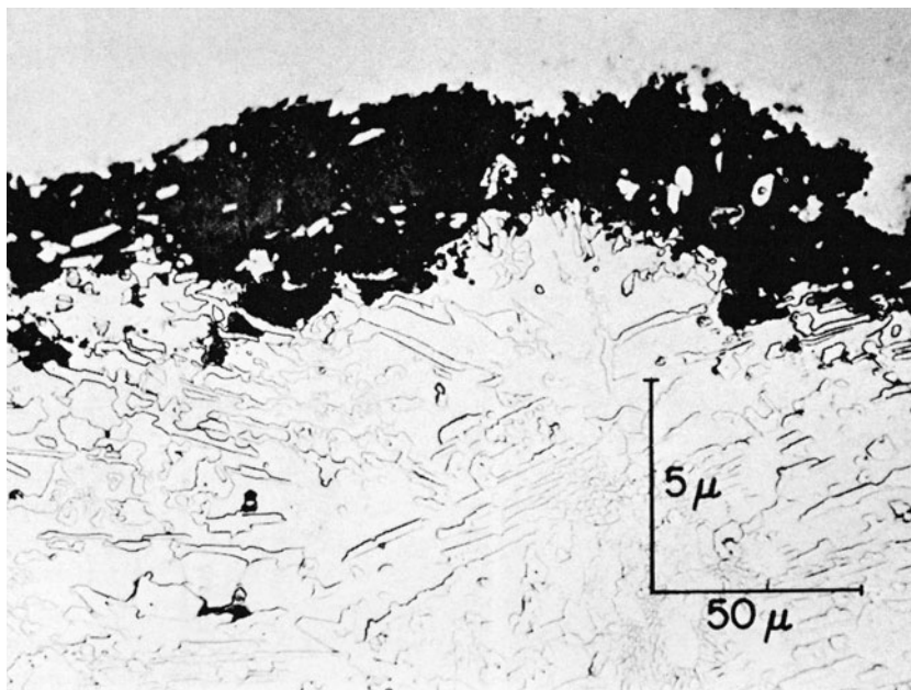
Fig. 14. Photomicrograph of taper section Martin-Wells material (area 2), showing clearly the oxide film.
