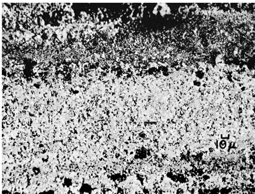
Fig. 15. Seating surface of Martin-Wells insert; the gray and dark gray areas indicate the continuous oxide film.
